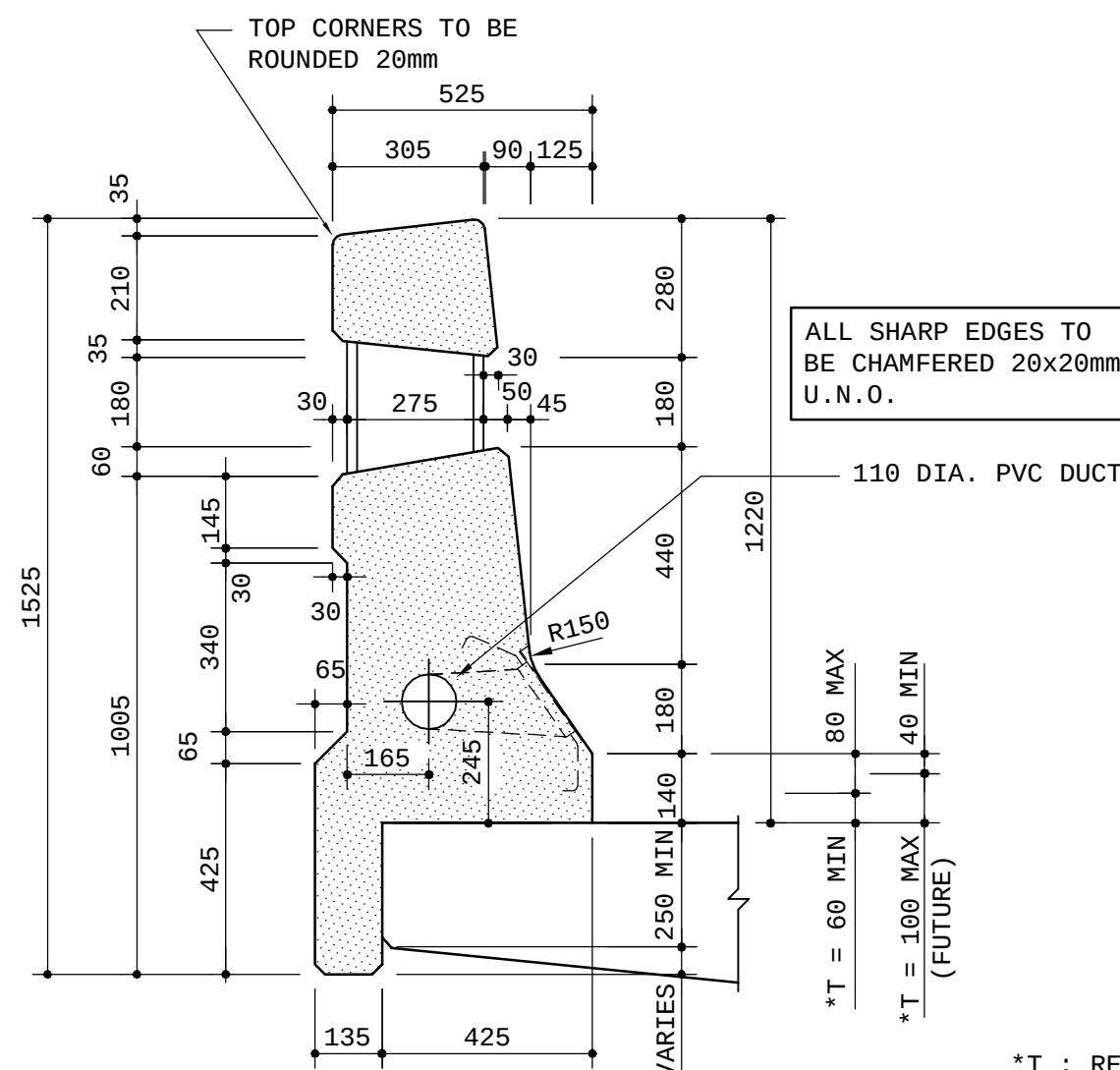
TYPICAL SECTION : TYPE A THROUGH PARAPET UNITS SCALE 1:15
