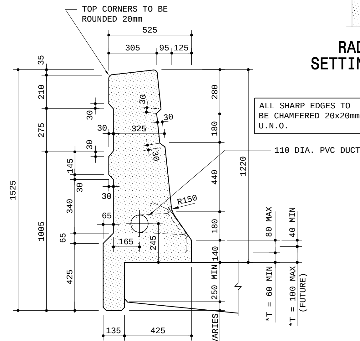
TYPICAL SECTION : TYPE B THROUGH PARAPET UNITS SCALE 1:15
